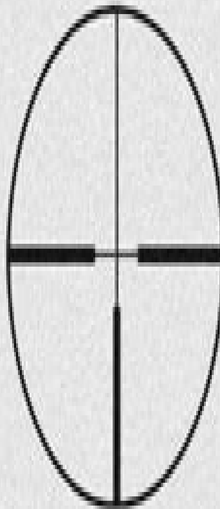
German #4 Reticle
