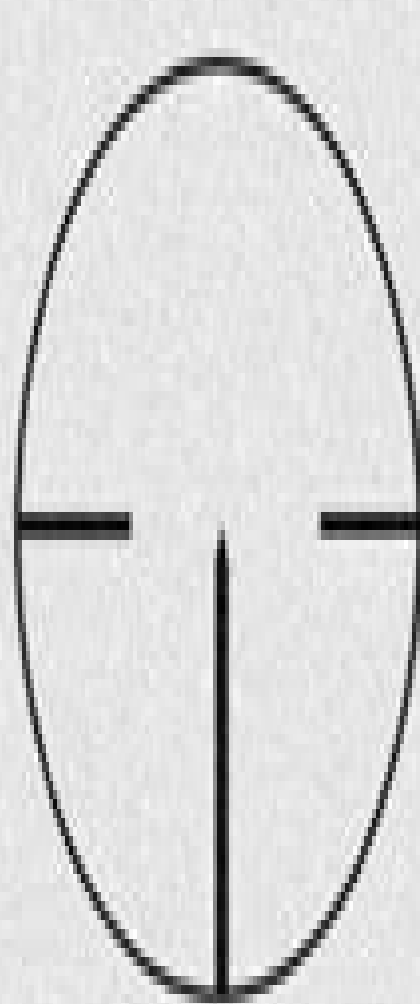
German #1 Reticle
